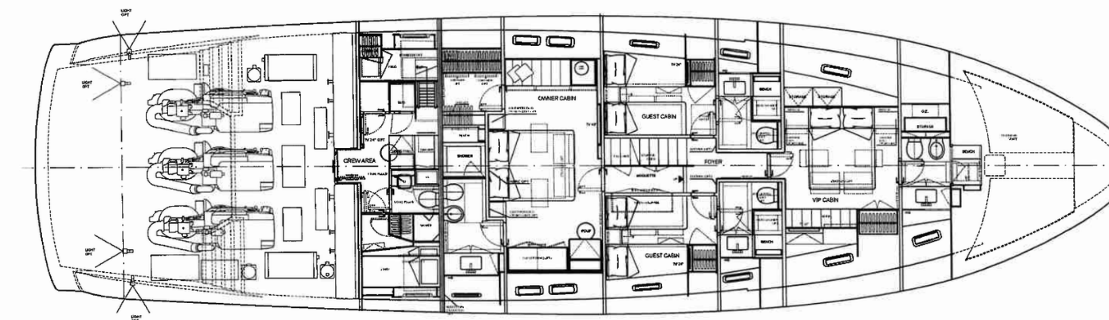
LOWER DECK
