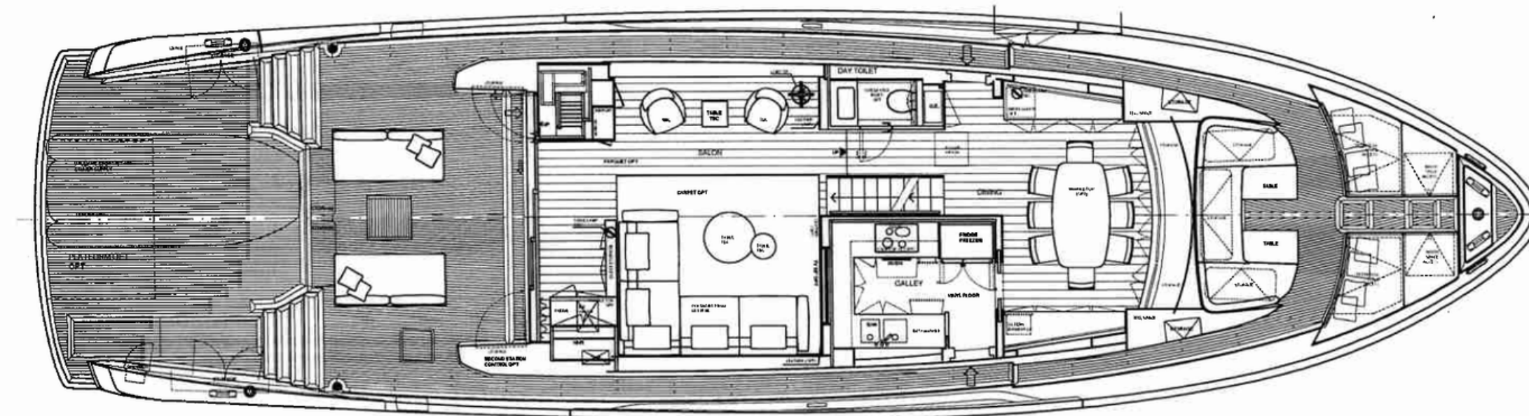
MAIN DECK
